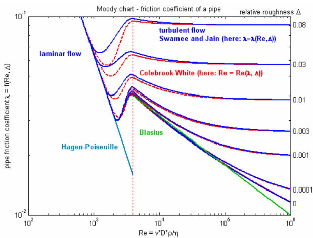
Figure 6. Moody Chart: \lg(\lambda) = f(\lg(\text{Re}), \Delta) , \zeta = \lambda L/D
